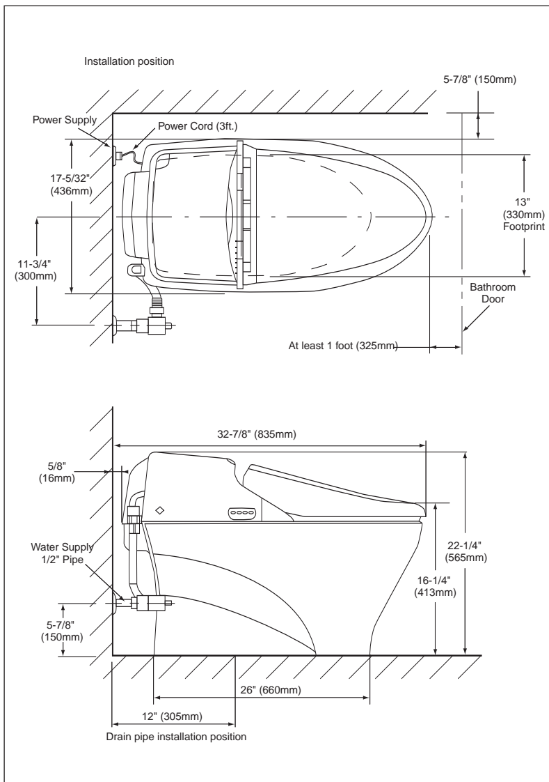
Neorest 600 MS990CG
